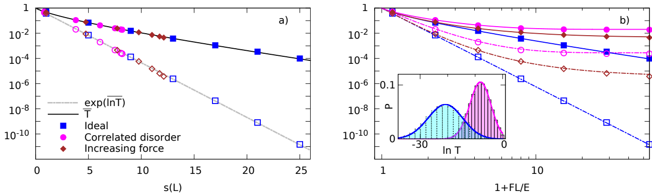
Figure 2. Analytical prediction vs numerical results for \overline{T} (solid lines and solid symbols) and \exp(\overline{\ln T}) (dashed-dotted lines and open symbols), for \alpha = 0.08 and 2mF/\hbar^2 k^3(0) = 0.01 in the following cases: uniform bias force and white-noise disorder (blue squares), uniform bias force and Gaussian correlated disorder with \sigma_R k(0) = 0.3 (magenta circles), harmonic bias force with 2m\omega/\hbar k(0)^2 = 0.01 and uncorrelated disorder (brown diamonds). Results plotted as a function of the metrics s(L) [for white noise and constant force, s(L) \propto \ln(1 + FL/E) ; see Eq. (4)]. (b) Results plotted as a function of 1 + FL/E . Inset: Probability distribution of \ln T for FL/E = 28 , as found from numerical simulations (histogram) compared to analytical prediction (line), for a constant force, with correlated (dark, magenta) and uncorrelated (light, blue) disorder.
