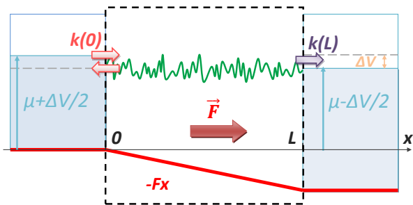
Figure 1. Transmission and conductance of a matter waveguide of length L (black rectangle) in the presence of a bias force F(x) and disorder (random green line). The bias field is shown for a constant force F and the reflected wave vectors are k(0) and the transmitted one is k(L) . The Landauer conductance is measured from the discharge between two reservoirs (left and right blue boxes) with average chemical potential \mu and infinitesimal potential difference \Delta V .
