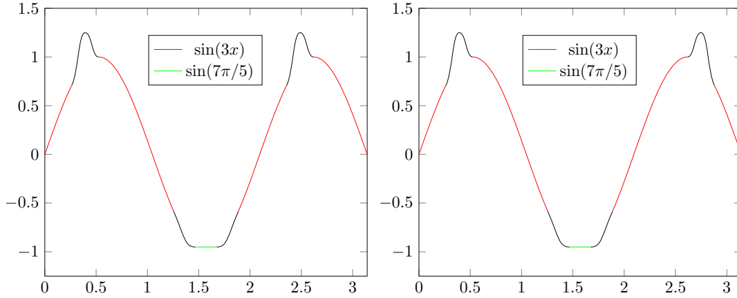
Figure 2: Examples of function \psi on [0, \pi]
