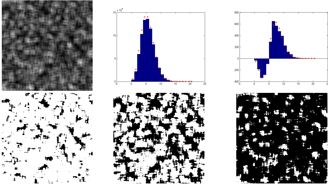
FIG 8. Shot noise random field with indicator functions of random squares. This sample has been obtained on a domain of size 2000 \times 2000 pixels, with a Poisson point process of intensity \lambda = 0.005 , and random squares of fixed side length R = 100 . Top middle and right figures: empirical Perimeter and Euler Characteristic as functions of the level t , compared with the theoretical value (red stars) of Equation (40). Bottom line: Three excursion sets corresponding respectively from left to right to the level t = 3 , t = 5 (that is the “critical level” where the Euler Characteristic turns from negative to positive) and t = 8 .
