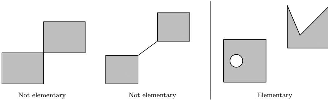
FIG 1. Left: two sets that are not elementary sets according to Definition 2: the boundary of the first set has one multiple point; for the second set, its boundary is not the union of disjoint piecewise C^2 Jordan curves. Right: an elementary set.
