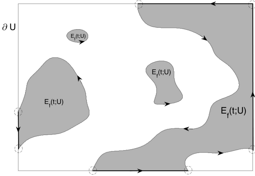
FIG 2. By the Gauss-Bonnet theorem, the Euler Characteristic of the excursion set E_f(t) \cap U (in gray) is equal to the total curvature of its boundary in the open rectangular domain U plus the turning angles at the points where \partial(E_f(t) \cap U) meets \partial U and also plus \pi/2 for each of the corners of the rectangle U that are in E_f(t) . All these special points are the ones marked by the small dashed circles on the figure.
