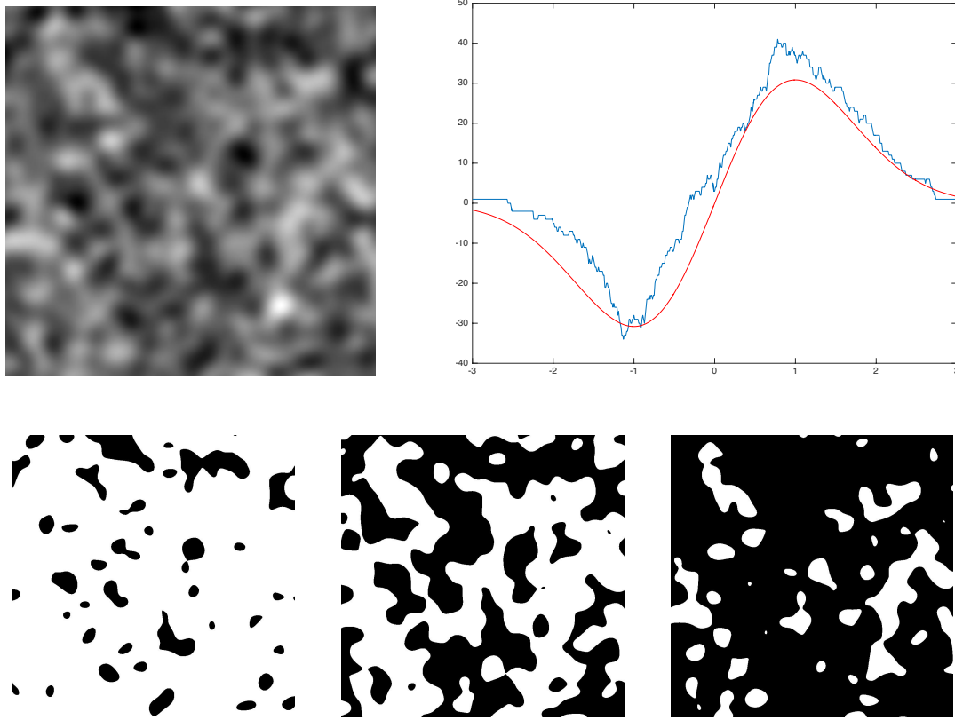
FIG 3. Gaussian random field with covariance \rho(x) = e^{-T^2 \|x\|^2} for T = 10 . This sample has been obtained using Matlab, with a discretized domain of size 2^{10} \times 2^{10} pixels, using the circulant embedding matrix method. Top right figure: empirical Euler Characteristic as a function of the level t (computed thanks to the Matlab function bweuler ), compared with the theoretical value (red curve) of Equation (9). Bottom line: Three excursion sets corresponding respectively from left to right to the level t = -1 , t = 0 (that is the “critical level” where the Euler Characteristic turns from negative to positive), and t = 1 .
