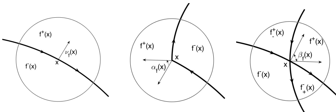
FIG 6. The three types of points of the discontinuity set of an elementary function. From left to right: a regular discontinuity point, a corner discontinuity point and an intersection discontinuity point.
