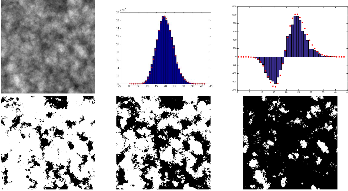
FIG 7. Shot noise random field with indicator functions of random disks. This sample has been obtained using Matlab, with a domain of size 2000 \times 2000 pixels, a Poisson point process of intensity \lambda = 0.001 , and random disks of radius R = 50 or R = 100 (each with probability 0.5). Top middle and right figure: empirical Perimeter and Euler Characteristic as a function of the level t (computed thanks to the Matlab functions bwperim and bweuler ), compared with the theoretical values (red stars) of Equation (37). Bottom line: Three excursion sets corresponding respectively from left to right to the level t = 15 , t = 19 (that is the “critical level” where the Euler Characteristic turns from negative to positive) and t = 25 .
