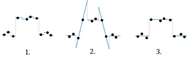
Fig. 4. Algorithm illustration on a simple step function: each point starts in its own set, then sets are iteratively merged together (starting with the closest ones), and finally artifacts at the frontiers between smooth components of F are removed and their point distributed into other models.
