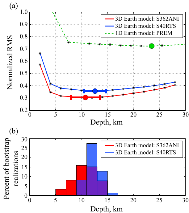
Figure 2. Centroid depth estimates in a 3-D Earth model for the 2015 Gorkha main shock. (a) Normalized RMS with respect to centroid depth. (b) Histogram of depth estimates from 5000 bootstrap realizations. Results are shown in red for S362ANI and in blue for S40RTS. Error bars in Figure 2a correspond to standard deviations estimated from 5000 bootstrap realizations presented in Figure 2b. Results obtained using the 1-D Earth model PREM are shown for reference in green.
