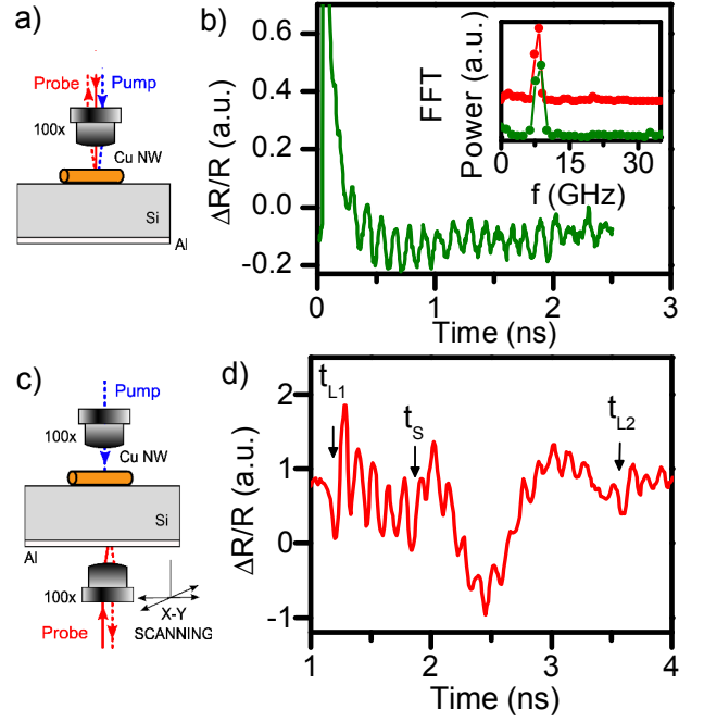
FIG. 2. (a) Front side configuration. Both the blue pump laser and the red probe laser are focused on a single 400 nm diameter copper nanowire using the same 100 \times objective with a numerical aperture NA = 0.95 . (b) Relative reflectivity \Delta R/R obtained in the front side configuration Figure 1a. It exhibits an oscillatory signal with a period T = 125 ps. Inset: normalized FFT power spectrum of the derived signal of Figure 2d (in red) and Figure 2b (in green). (c) Back side configuration. The two laser beams are focused on different sides of the silicon membrane. The probe is mounted on a piezoelectric stage in order to map the displacement field on a maximum 150 \mu\text{m} \times 150 \mu\text{m} area. (d) Relative reflectivity \Delta R/R obtained in the back side configuration Figure 1c. It exhibits an oscillatory component with a period T = 125 ps.
