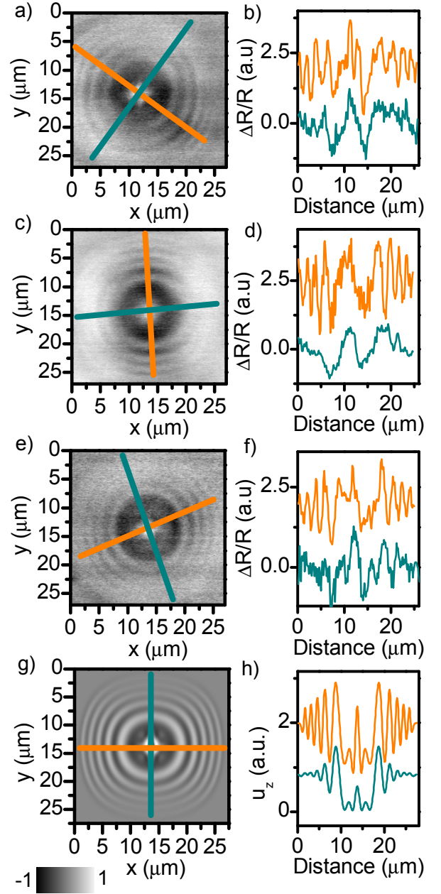
FIG. 5. (a),(c) and (e) Two-dimensional x-y surface displacement mapping 700 ps after the longitudinal echo detection on the central position with a \times 50 objective. The three different underlying nanowires are oriented along the blue cyan line. (g) FDTD two-dimensional x-y surface displacement ( u_z ) mapping 700 ps after the longitudinal echo detection on the central position. The acoustic source is \sim 2 \mu\text{m} wide along the blue cyan line and \sim 0.2 \mu\text{m} wide along the orange line. (b), (d), (f) and (h) Surface displacement profile, respectively along the orange and the cyan line. The offset is for readability purpose.
