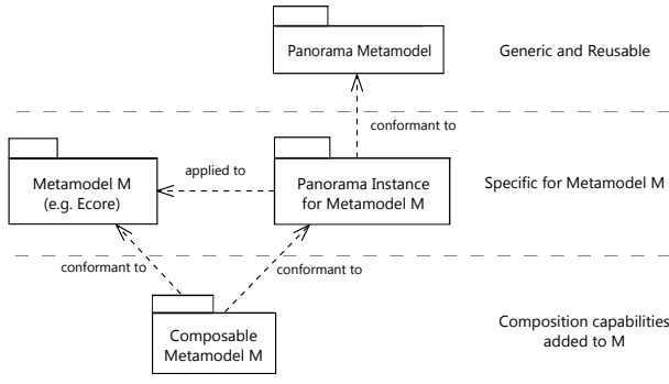
Figure 4. Adding composition capabilities to a Metamodeling language
