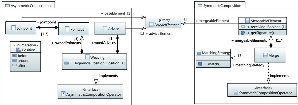
Figure 2. Panorama Composition Framework - Applied to Ecore
