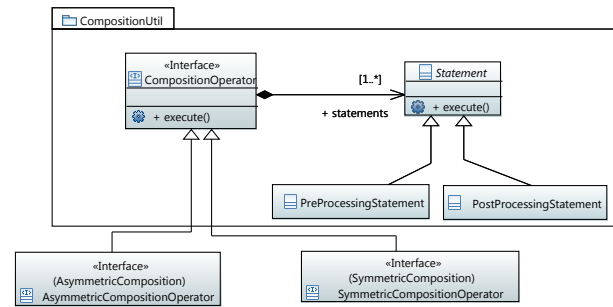
Figure 3. CompositionUtil Package
