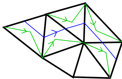
FIGURE 12. What happens inside the cusp: c in blue and g \circ h(c) in green.
