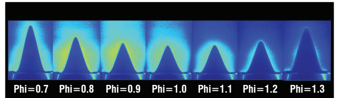
Figure 7 - Evolution of the structure of the laminar flame of a premixed kerosene/air combustion for various equivalence ratios. P=0.5 MPa, T_{air}=400 K.
