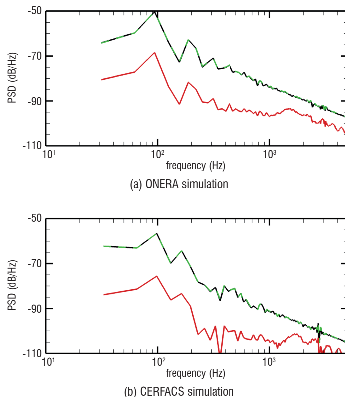
Figure 21 - Spectra of the acoustic invariants leaving the nozzle — P_1^- from CFD; - - - P_1^- from analytical methods; — P_2^+ from analytical methods
