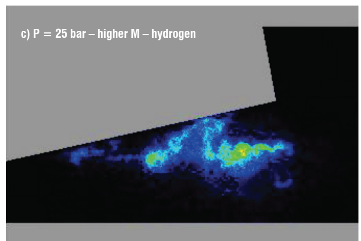
Figure 13 – Instantaneous PLIF images of OH radical concentration
