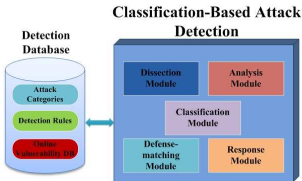
Fig. 1. AIDD Architecture
