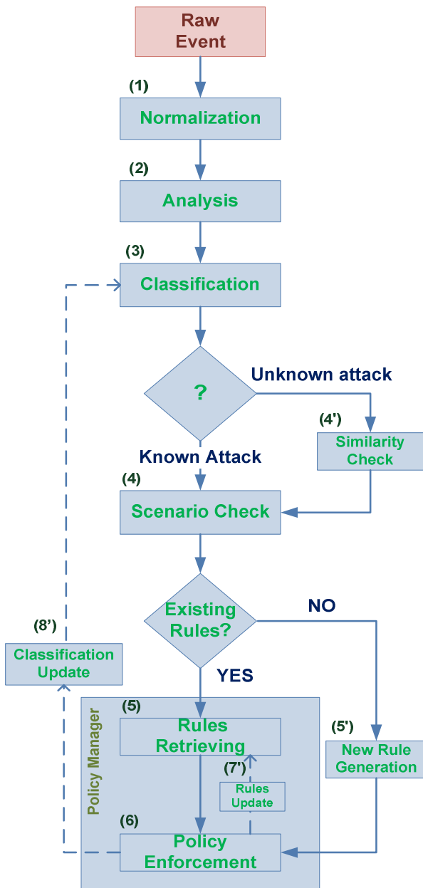
Fig. 5. Architecture Workflow
