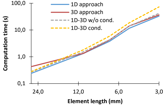
Figure 20: Computation times for the prestressed concrete volume (linear elastic regime).
