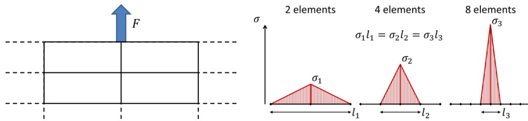
Figure 2 : Illustration of the stress concentration effect with a 2D material problem for a given nodal force.
