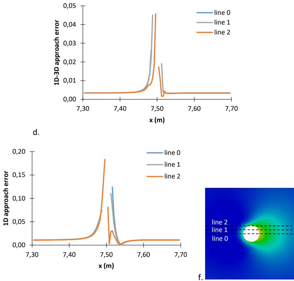
Figure 14: Values of the equivalent strain in the concrete on horizontal lines (f) of the cross-section
