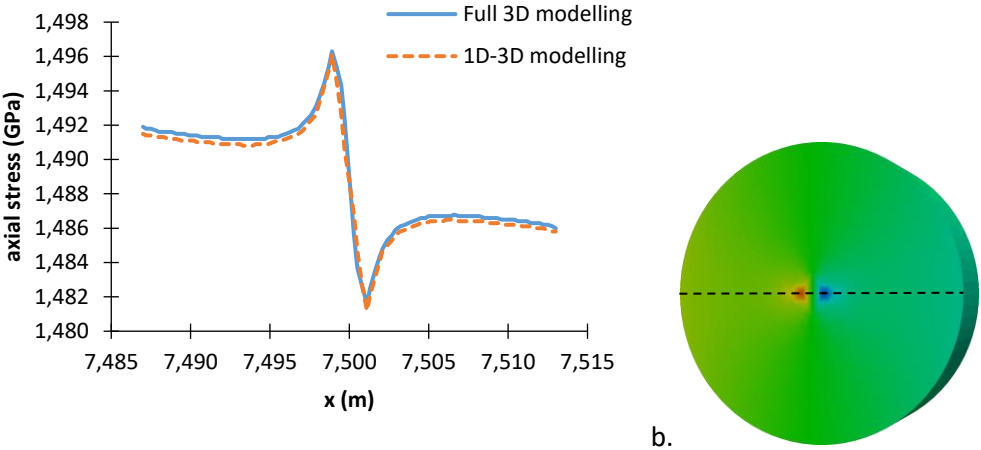
Figure 6: Longitudinal stress in the tendon after computation of the equivalent forces (a), along a line (b).
