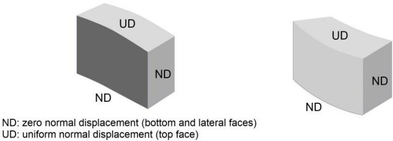
Figure 24 : Boundary conditions and loading applied to the RSV [10].
