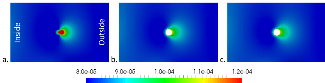
Figure 11: Equivalent strain distributions on the curved concrete volume: 1D modelling (a), 1D-3D modelling (b) and 3D modelling (c).
