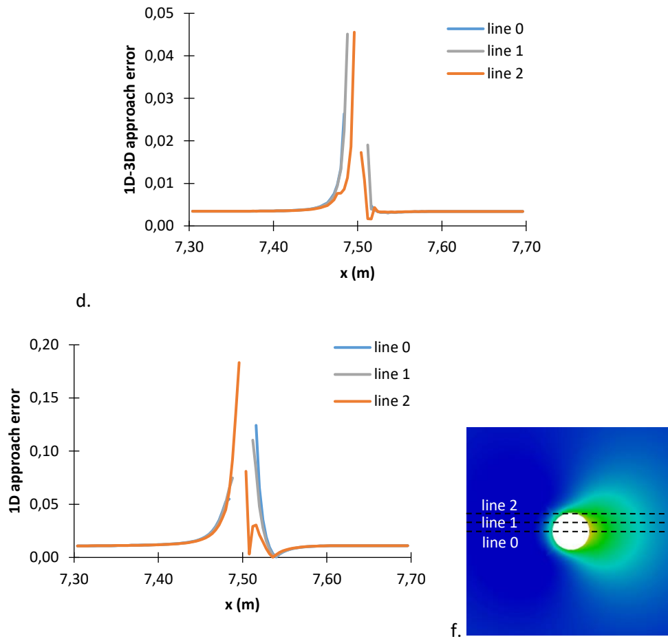
Figure 14: Values of the equivalent strain in the concrete on horizontal lines (f) of the cross-section (a: line 0, b: line 1, c: line 2, d: error map on the three lines with the 1D-3D approach, e: error map on the three lines with the 1D approach (f). The error estimation requires a projection in this case).
