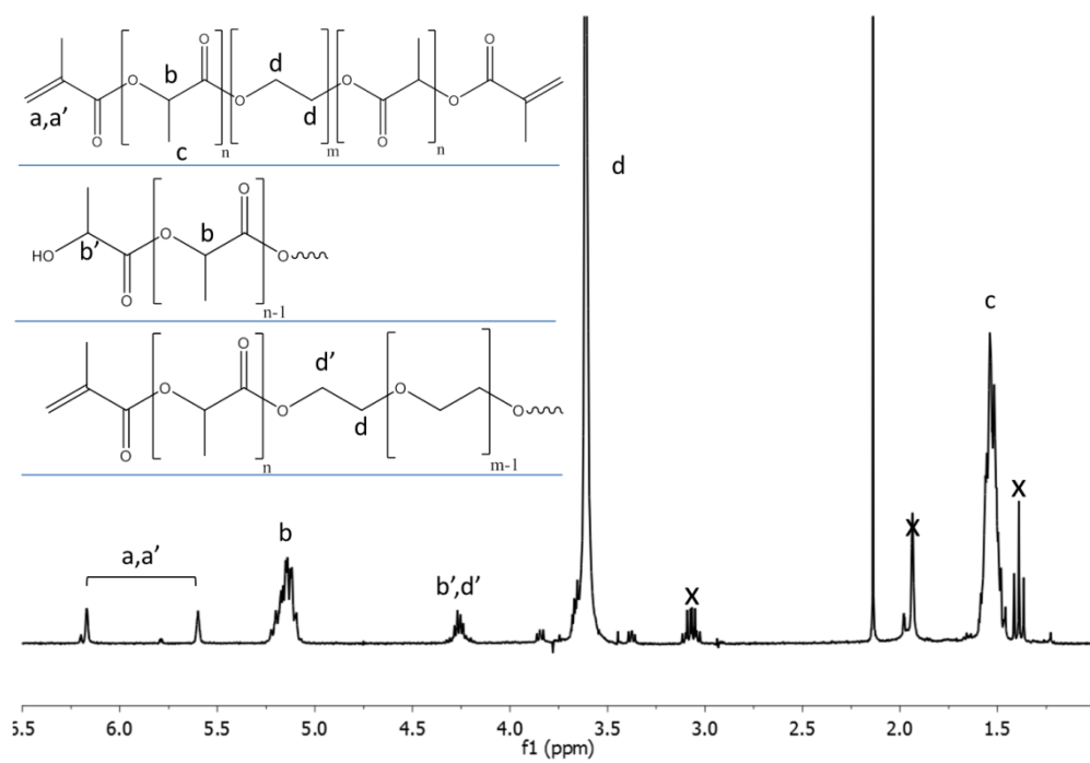
Figure S1. ^1\text{H} NMR (300 MHz; \text{CDCl}_3 ) of methacrylated \text{PLA}_9\text{-PEG}_{2k}\text{-PLA}_9 copolymer. Crosses correspond to residual solvents and triethylammonium salt.
