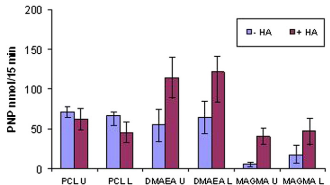
Fig. 10. Alkaline phosphatase in situ assay on MSC grown for seven days.
