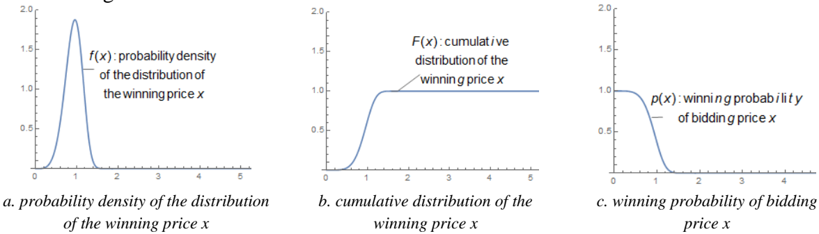
Fig2 Winning probability submitted to Weibull Distribution
