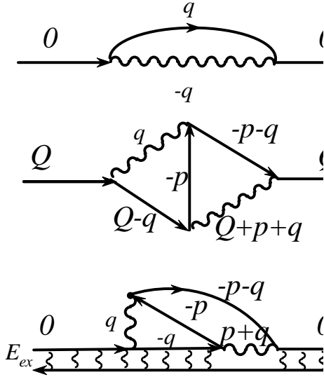
Figure 2: (a) Feynman diagram which describes the electron energies. (b) The second order energy correction to the electron state. (c) The self-energy correction to the exciton state (d line connected by the wavy Coulomb lines) interaction, obtained from diagram (b) at Q are the electron and hole Green functions, \Gamma the exchange vertexes.
