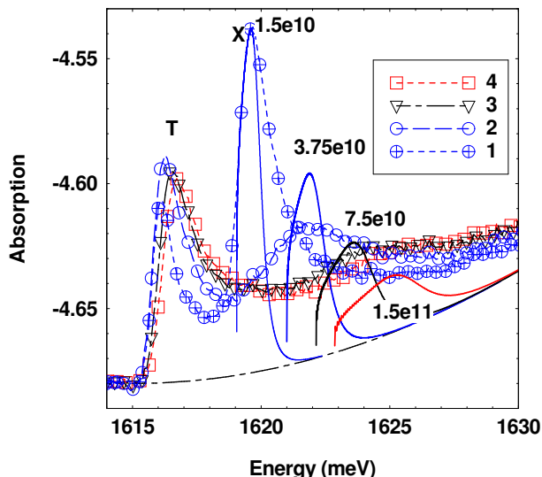
Figure 5: (Color online) Curves (1-4) are the experimental data on absorption of a 10 nm CdTe(0.3%Mn) single quantum well in zero magnetic field at different free electron concentrations. A resonance peak (T) corresponds to creation of the singlet trion appearing below the exciton resonance (X). Solid curves are the calculated exciton line profiles at free electron densities of 1.5, 3.75, 7.5, and 15.0 \cdot 10^{10} \text{ cm}^{-2} . The dashed curve is a background added to the calculated spectra.
