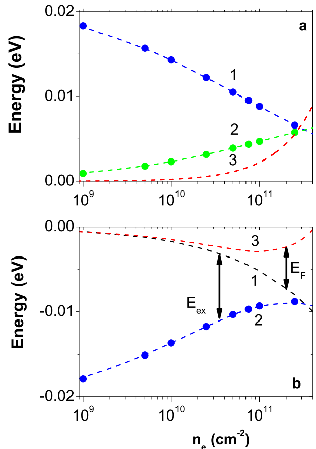
Figure 1: (Color online) (a) Curve (1) presents the dependence of the absolute value of the exciton binding energy on the free electron concentration for a 10 nm wide CdTe quantum well, taking into account only the static screening. Curve (2) presents the repulsive phase-space filling correction decreasing the exciton binding energy, and Curve 3 is the absolute value of the Fermi energy. (b) Curve (1) is the rigid shift of the band gap E_G corresponding to diagram (a) of Fig.2. Curve (2) is the exciton binding energy with respect to E_G as a function of the electron concentration taking into account the static screening and phase-space filling effects. Curve (3) is the Fermi energy with respect to E_G .
