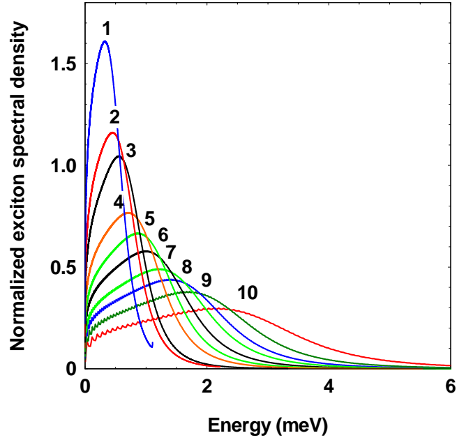
Figure 3: (Color online) Broadening and shift of the normalized to unity, spectral density of the exciton ground state caused by the second order exchange interaction for ten electron concentrations in a 10 nm CdTe/CdMgTe quantum well. The zero of energy corresponds to the exciton ground state at zero temperature and zero electron concentration. The ten electron concentrations expressed in 10^{10} \text{ cm}^{-2} are equal to 0.5, 1.0, 1.5, 2.5, 3.75, 5.0, 7.5, 10.0, 15.0, and 25.0.
