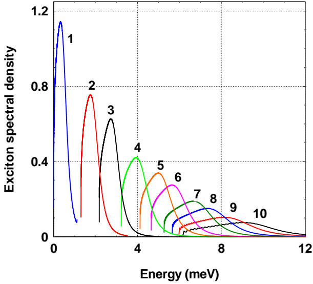
Figure 4: (Color online) Spectral density of the exciton ground state for a 10 nm CdTe/CdMgTe quantum well parameters at increasing electron concentration. The zero of energy corresponds to the exciton ground state at zero temperature and electron concentration equal to 0.5 \cdot 10^{10} \text{ cm}^{-2} . As compared to Fig. 3, the threshold energy of each exciton band is shifted upwards: Here, in addition to the second order shift and broadening due to exchange interaction, the static screening, the first-order rigid shift due to exchange interaction, the phase-space filling effect, and the decrease of the oscillator strength are all taken into account. The ten electron concentrations expressed in units of 10^{10} \text{ cm}^{-2} are equal to 0.5, 1.0, 1.5, 2.5, 3.75, 5.0, 7.5, 10.0, 15.0, and 25.0.
