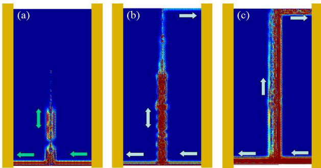
FIG. 8. Local density of injected electrons in the 200 nm wide ribbon with a 5-8 line defect and Anderson disorder of strength W=2 eV along the defect at energy 100 meV (a), 200 meV (b) and 300 meV (c).
