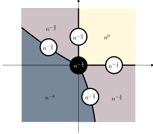
Figure 7: The universality classes as a function of drift for the centrally weighted family of the Tandem model given by (40): (1, 0) \rightarrow a , (-1, 1) \rightarrow a^{-1}b , (0, -1) \rightarrow b^{-1} .
