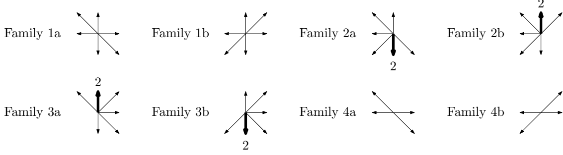
Figure 5: Equivalence class representatives corresponding to the families of walks with D -finite generating functions given by Kauers and Yatchak [29]; unlabeled steps have weight 1.
