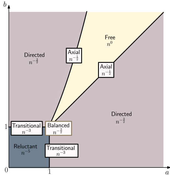
Figure 2: The polynomial growth ( n^{-\alpha} in Theorem 1) for the weighted GB model given as a function of the weight parameters a and b . Each region corresponds to a universality class. The boundaries of the 2-dimensional regions, and their intersection form distinct regions.
