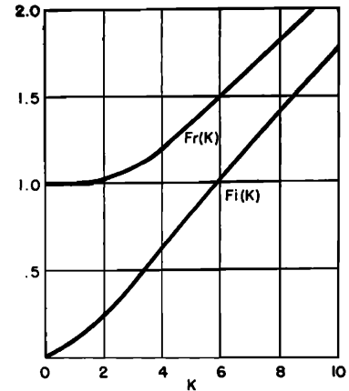
FIG. 4. Frequency correction functions for the viscosity in three-dimensional flow.
