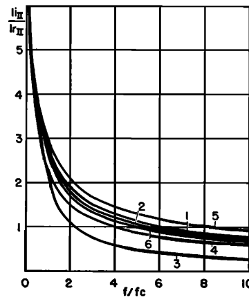
FIG. 14. Attenuation coefficient of dilatational waves of the second kind.
