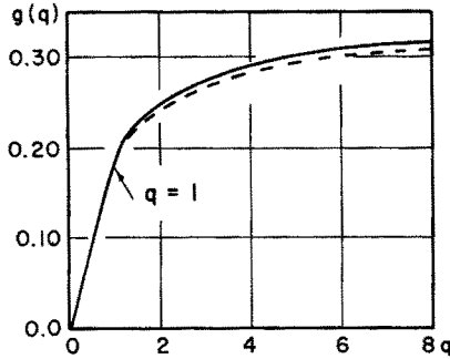
FIG. 2. Plot of g(q) for the velocity profile of Fig. 1(a). The dotted line shows the value of the approximate expression g(q) = 289/(73 + 81q) for q > 1 .
