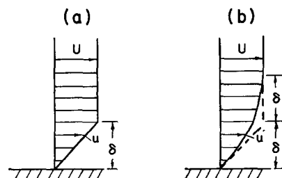
FIG. 1. Idealized velocity profiles for laminar boundary layers. (a) piece-wise linear profile; (b) parabolic profile.
