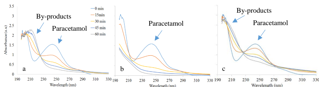
Figure 2. Absorption spectra in function the composition of the injected gas a) air ( U = \pm 6.8 kV); b) 90% Ar + 10% O 2 ( U = \pm 5 kV); c) 90% Ar + 10% air ( U = \pm 3.6 kV).
