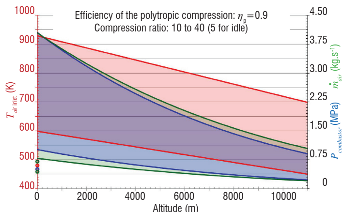
Figure 21 – Flight envelope conditions targeted with the MICADO test rig
