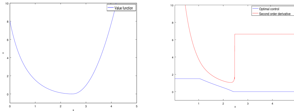
Figure 1: (Example 1) Left: Plot of the value function at time t = T . Right: Optimal control (blue) at time t = T , and plot of v_{xx}(T, \cdot) (red).
