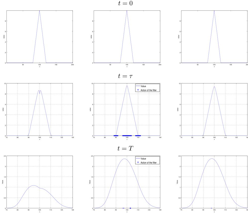
Figure 4: (Example 2) From top to bottom: value function at t = 0 (the payoff), after one time-step t = \tau , and at terminal time t = T . From left to right: CN scheme, CN+filter scheme, BDF scheme.
