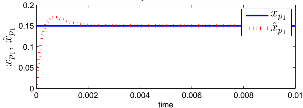
Asymptotic stability of the closed loop system
