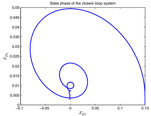
Fig. 4. Phase portrait of the state x_p .
