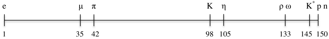
Fig.1. N(j) for elementary particles from electron to neutron
