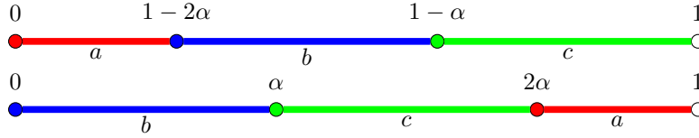
Figure 3.1: A 3-interval exchange transformation.
