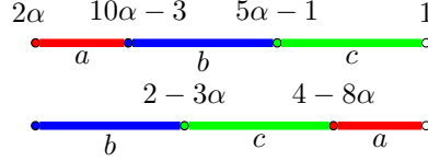
Figure 4.4: The transformation S .
