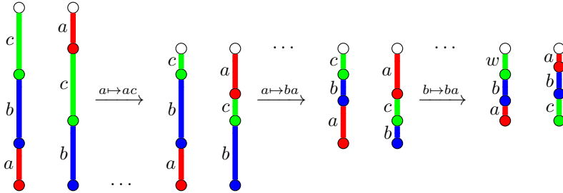
Figure 4.7: The sequence \chi \in \{\varphi, \psi\}^*
