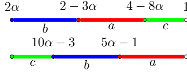
Figure 4.5: The transformation U .
