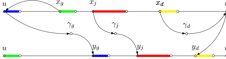
Figure 3.6: The transformation induced on [u, v[ .
