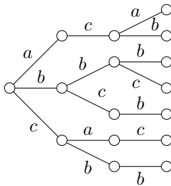
Figure 2.1: The words of length \leq 3 of \mathcal{D}_f(F) .
