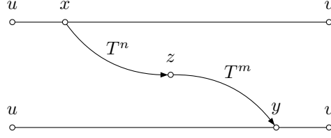
Figure 3.5: The neighbors of z with respect to I = [u, v[ .
