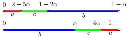
Figure 4.3: The transformation \psi^2(T) .
