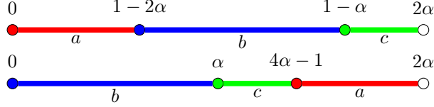
Figure 3.4: The transformation induced on I .
