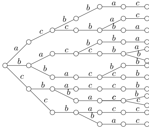
Figure 3.3: The words of length \leq 6 of the set F .
