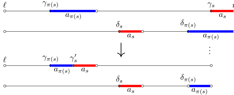
Figure 4.2: Case 1 in Rauzy induction.
