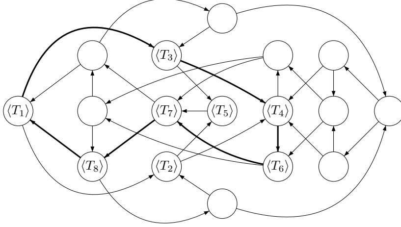
Figure 5.1: Modified induction graph of the transformation T .
