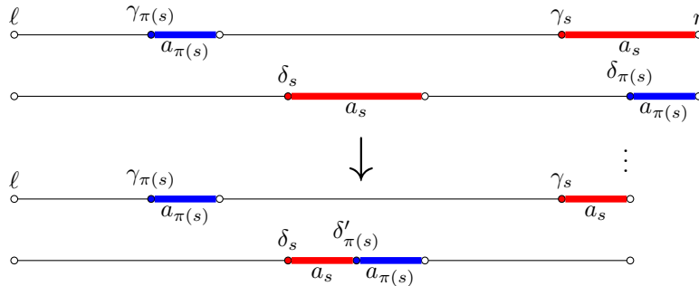
Figure 4.1: Case 0 in Rauzy induction.
