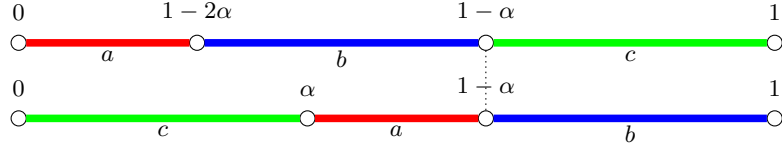
Fig. 3. A 3-interval exchange transformation.
