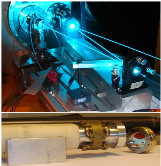
Fig. 7 (Upper) Intracavity laser beam of the \text{Ar}^+ laser operating in a Z-fold extended cavity mode of 10 m long. The output coupler of the \text{Ar}^+ laser, which can be seen close to one of the intracavity guiding mirrors, has been replaced by another one with a curvature radius of 10 m. (Lower) New used output coupler of 2 inch of diameter and 99.55% of reflectivity. It has been mounted on the mole supporting structure, which has been inserted inside the magnet aperture to operate the \text{Ar}^+ laser in extended cavity mode.
