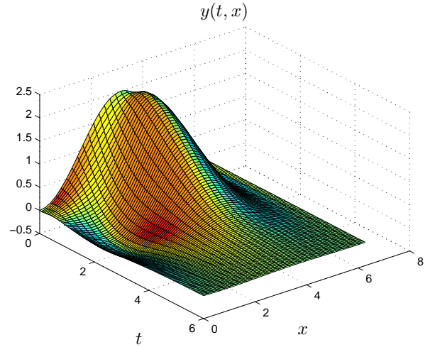
FIG. 7. Solution y(t, x) with a localized feedback law saturated; u_0 = 0.5
