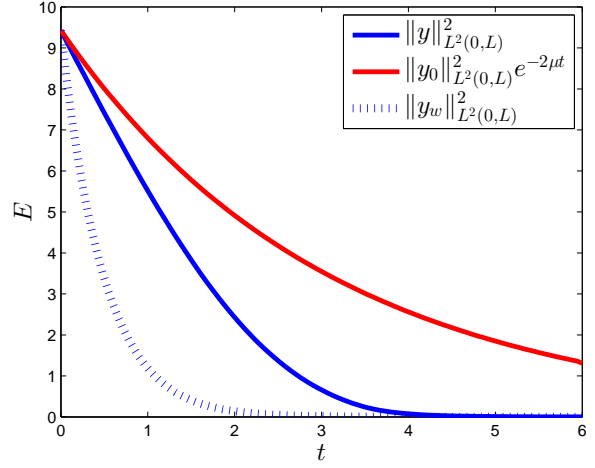
FIG. 5. Blue: Time evolution of the energy function \|y\|_{L^2(0,L)}^2 with a saturation u_0 = 0.5 and a_0 = 1 . Red: Time evolution of the theoretical energy \|y_0\|_{L^2(0,L)}^2 e^{-2\mu t} . Dotted line: Time evolution of the solution without saturation y_w and a_0 = 1 .
