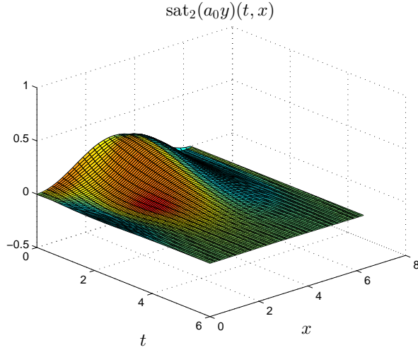
FIG. 4. Control f = \text{sat}_2(a_0 y)(t, x) where \omega = [0, L] , u_0 = 0.5
