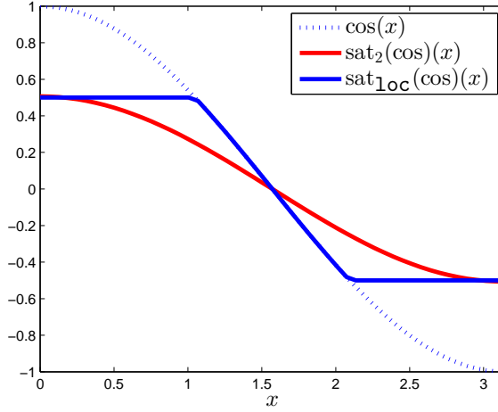
FIG. 1. x \in [0, \pi] . Red: \text{sat}_2(\cos)(x) and u_0 = 0.5 , Blue: \text{sat}_{1oc}(\cos)(x) and u_0 = 0.5 , Dotted lines: \cos(x) .
