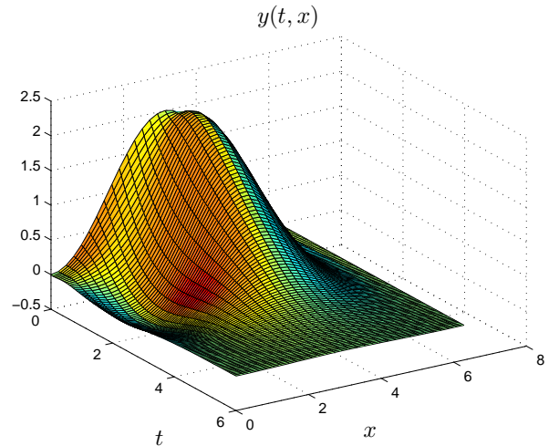
FIG. 3. Solution y(t, x) with the control f = \text{sat}_2(a_0 y) where \omega = [0, L] , u_0 = 0.5
