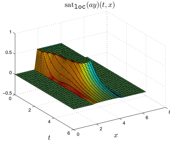
FIG. 8. Control f = \text{sat}_{\text{loc}}(ay)(t, x) where \omega = [\frac{1}{3}L, \frac{2}{3}L] , u_0 = 0.5
