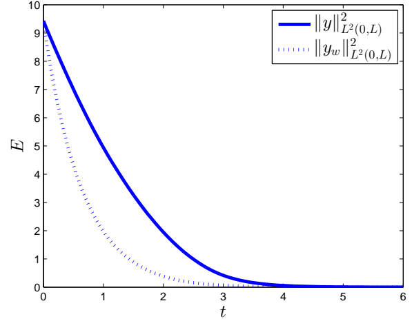
FIG. 9. Blue: Time evolution of the energy function \|y\|_{L^2(0,L)}^2 with a saturation u_0 = 0.5 , a_0 = 1 and \omega = [\frac{1}{3}L, \frac{2}{3}L] . Dotted line: Time evolution of the solution without saturation y_w with a_0 = 1 and \omega = [\frac{1}{3}L, \frac{2}{3}L] .
