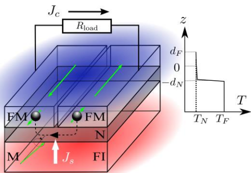
Figure 1 – Spin Seebeck thermoelectric generator [14]. A spin current is generated by the temperature difference between a ferromagnetic insulator FI and normal metal N with weak spin dissipation. The spin accumulation in N is detected by metallic ferromagnetic contacts (FM) with antiparallel magnetizations collinear to that of FI. The spin Seebeck voltage can carry out useful work by generating a charge current through a load resistance.
