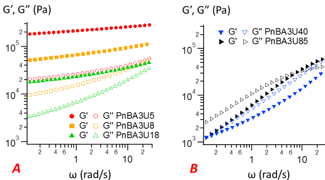
Figure 9: Linear rheology curves at 25°C for low (A) and high (B) molecular weight PnBA3U. The storage modulus G' is represented by filled markers, the loss modulus G'' by unfilled markers (data from previous works 1 ).
