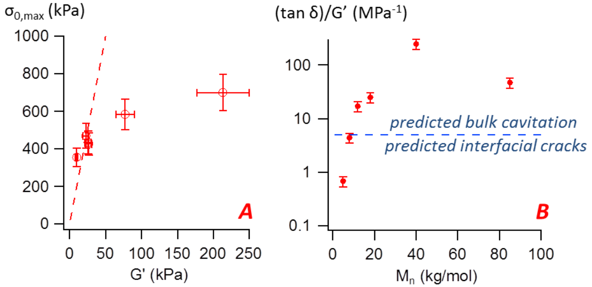
Figure 10: (A) variation of the maximal nominal stress \sigma_{0,max} with the storage modulus G'(\omega_c) measured at the representative angular frequency \omega_c = 2\pi V_{deb}/h_0 = 6.28 rad/s (the dashed line represents \sigma_{0,max} = 20G'(\omega_c) ), (B) variation of the ((\tan \delta)/G')(\omega_c) ratio with the molecular weight for the PnBA3U materials. The straight line represents the constant C proposed by Deplace et al. 32 to predict debonding by interfacial cracks or by bulk cavitation.
