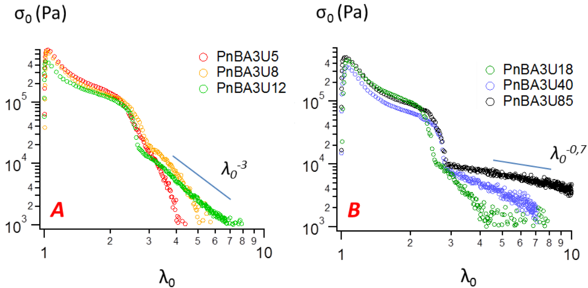
Figure 5: Probe-tack curves for low (A) and high (B) molecular weight PnBA3U polymers at room temperature (traction speed 100 \mu\text{m}/\text{s} ).
