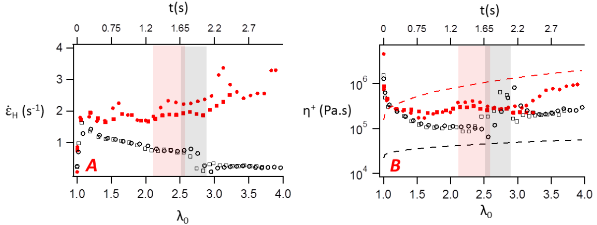
Figure 14: Variation of the Hencky strain rate (A) and the local extensional viscosity (B) with the nominal strain and time for PnBA3U5 and PnBA3U85. The highlighted regions corresponds to the phase of the equilibration of pressure, where \dot{\epsilon}_H and \eta^+ are scattered and thus, difficult to interpret. Two experimental curves are shown for each material. In the graph 13.B, the red and black dashed lines are the limiting linear viscoelastic extensional viscosities of PnBA3U5 and PnBA3U85, respectively.
