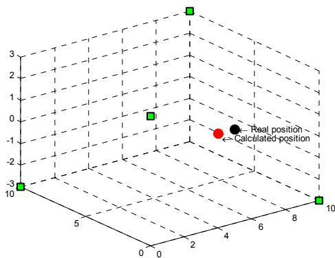
Figure 1 Resulting position with TOA method
