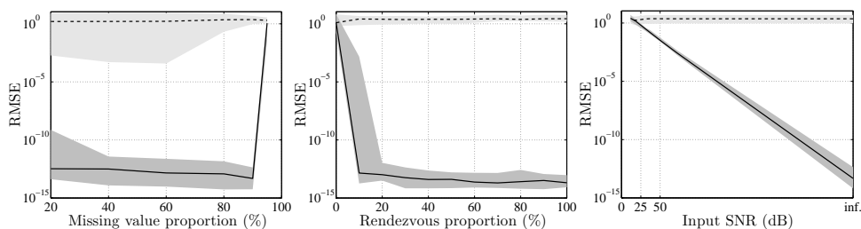
Fig. 2. Performance of the BMSC method vs ( left ) the proportion of missing values, ( center ) the proportion of rendezvous between calibrated and uncalibrated sensors, and ( right ) the input SNR.
