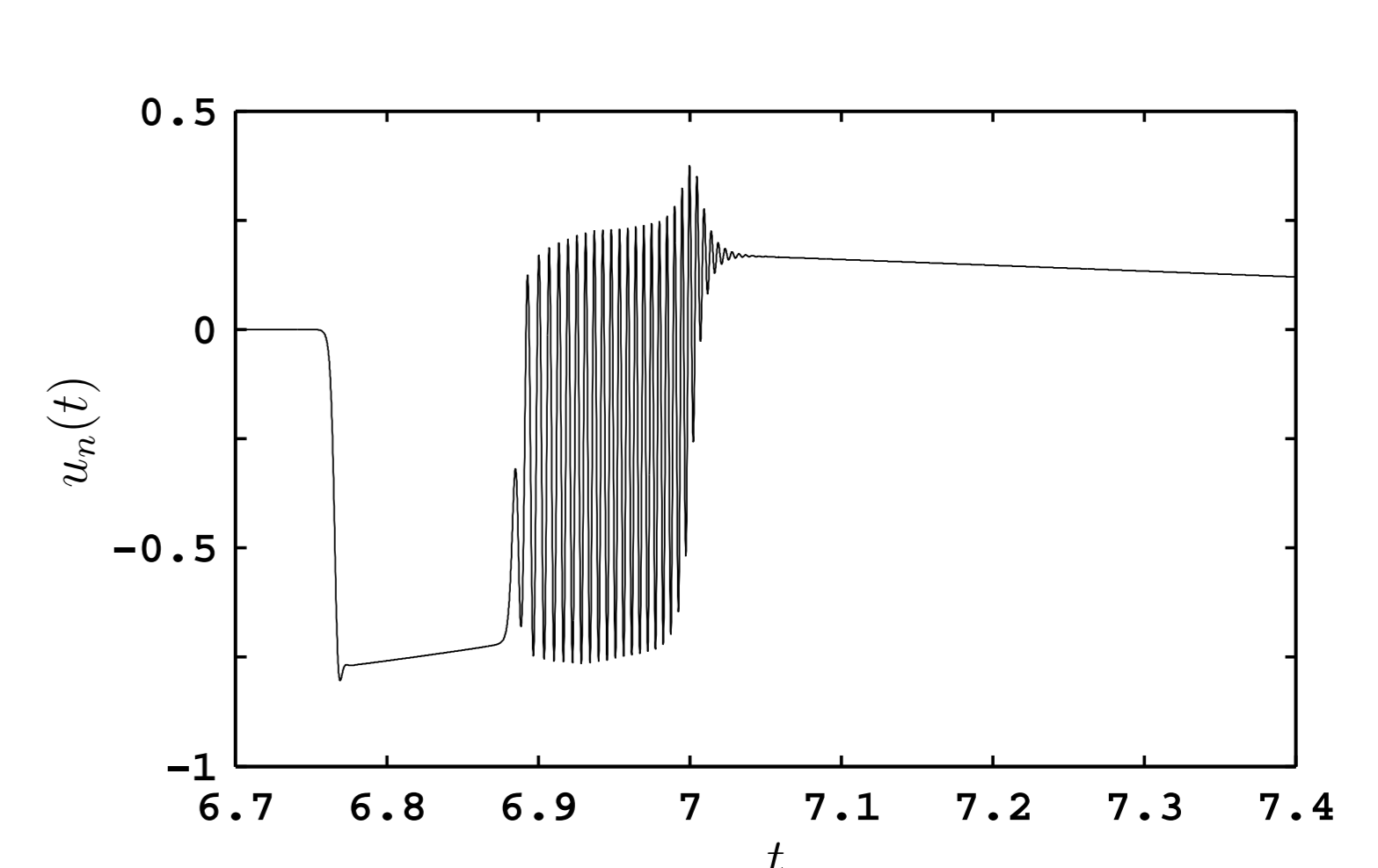
Fig. 11: Velocity u_n(t) at n = 17500
