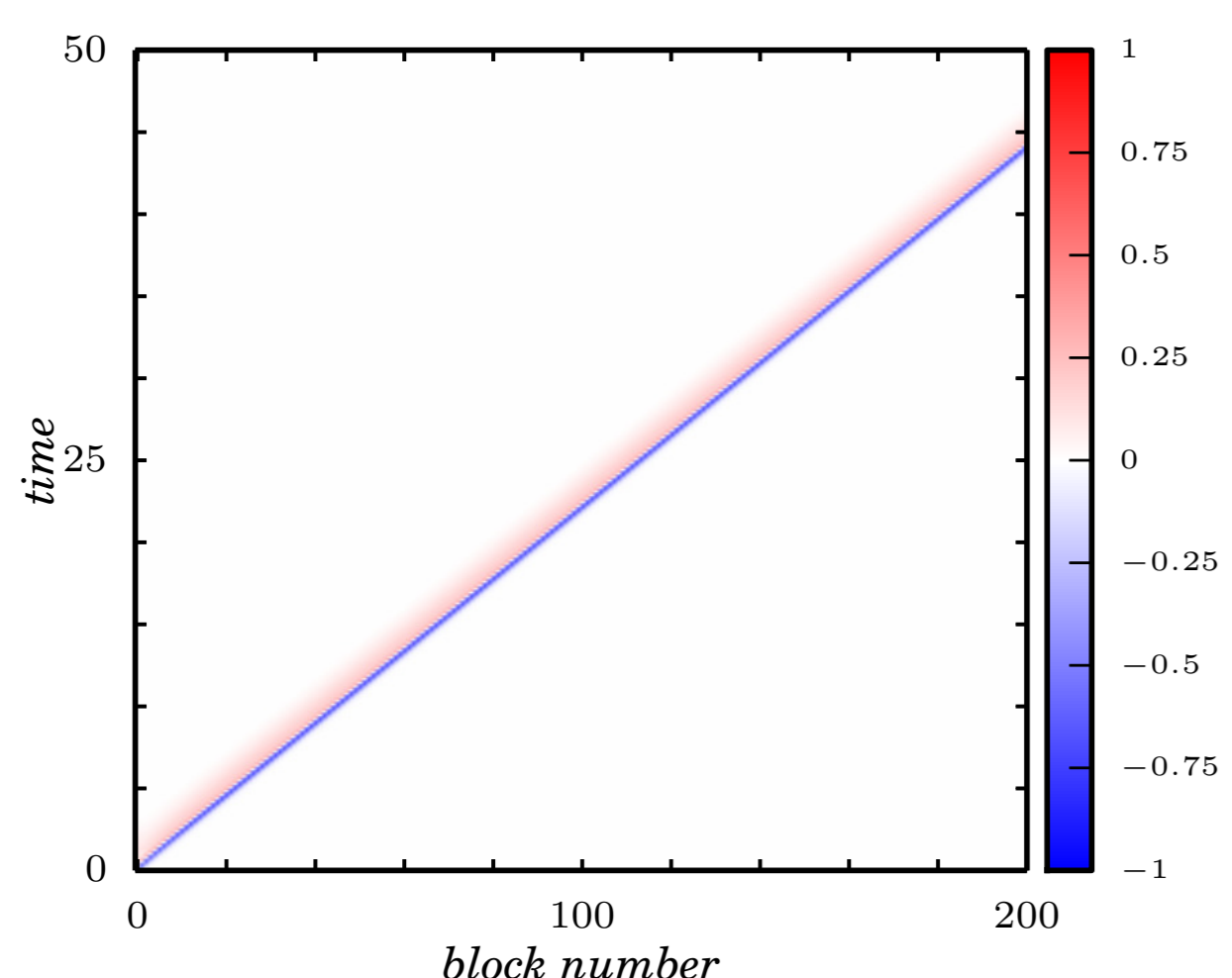
Fig. 8: Velocities u_n(t) .
