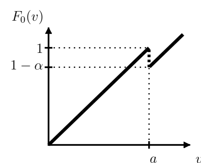
Fig. 4: Non-smooth friction function.
