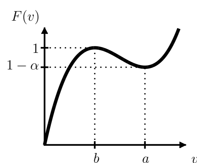
Fig. 3: Smooth friction function.
