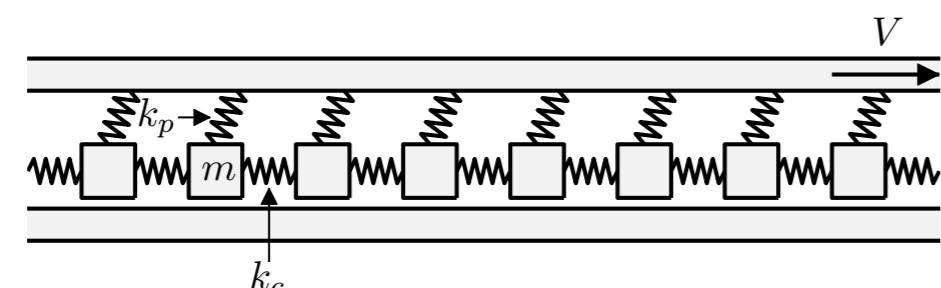
Fig.1 Schematic view of the Burridge-Knopoff model
