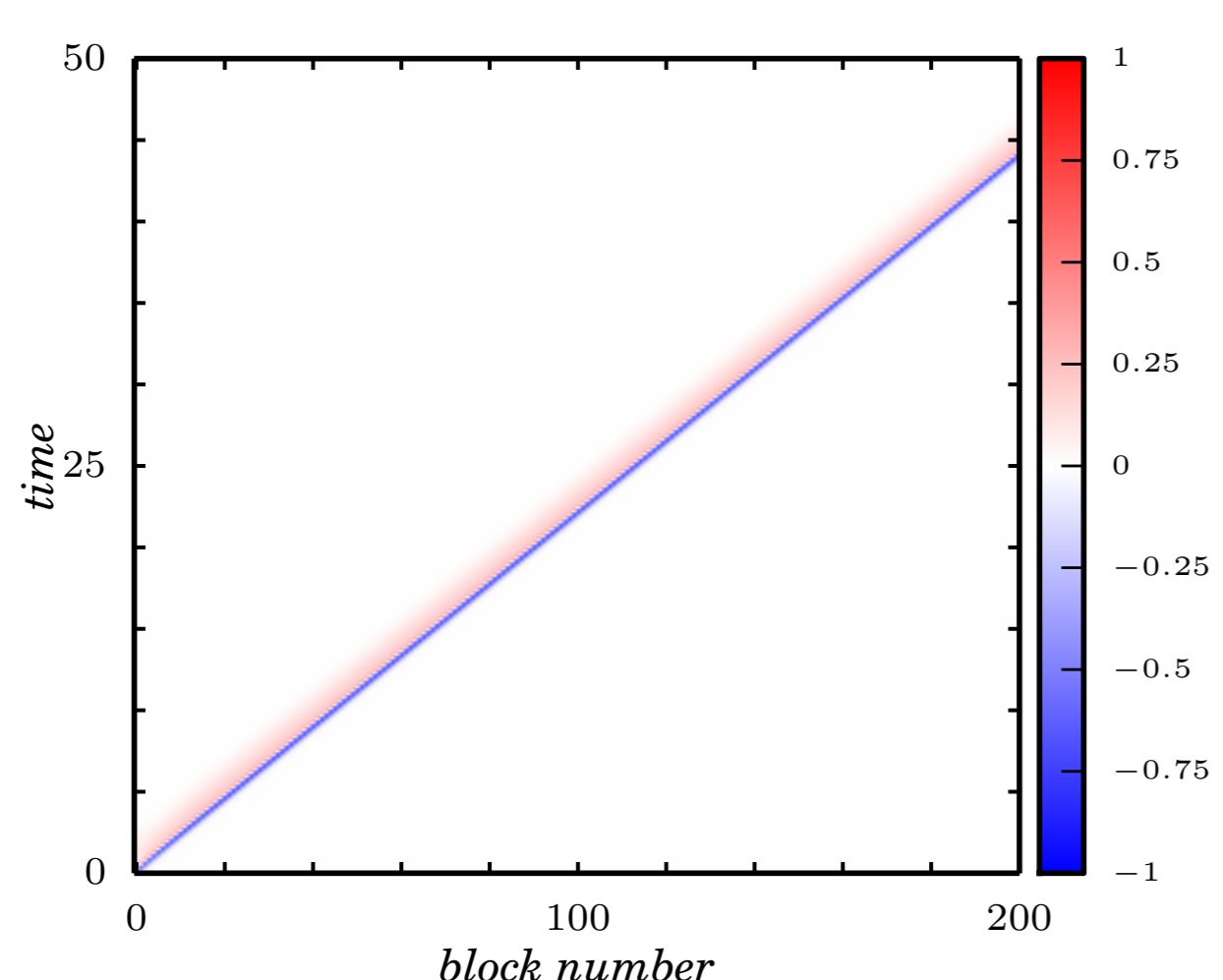
Fig. 8: Velocities u_n(t) .
