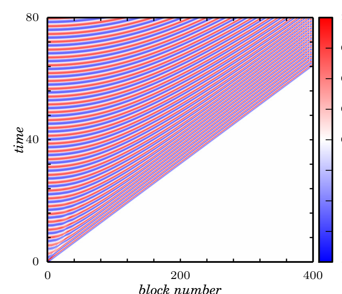
Fig. 10: Velocities u_n(t) .
