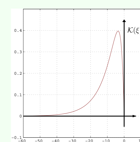
Fig. 5: Shape of function \mathcal{K}(\xi)
