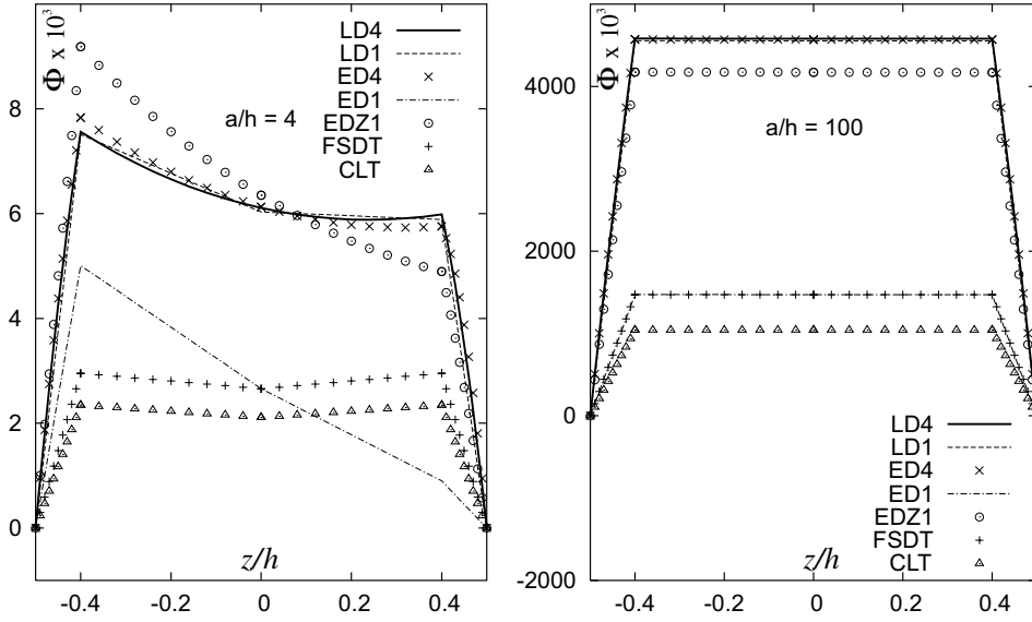
Fig. 13. Problem II, potential \Phi \times 10^3 vs. z/h for ah = 4 and ah = 100 .
