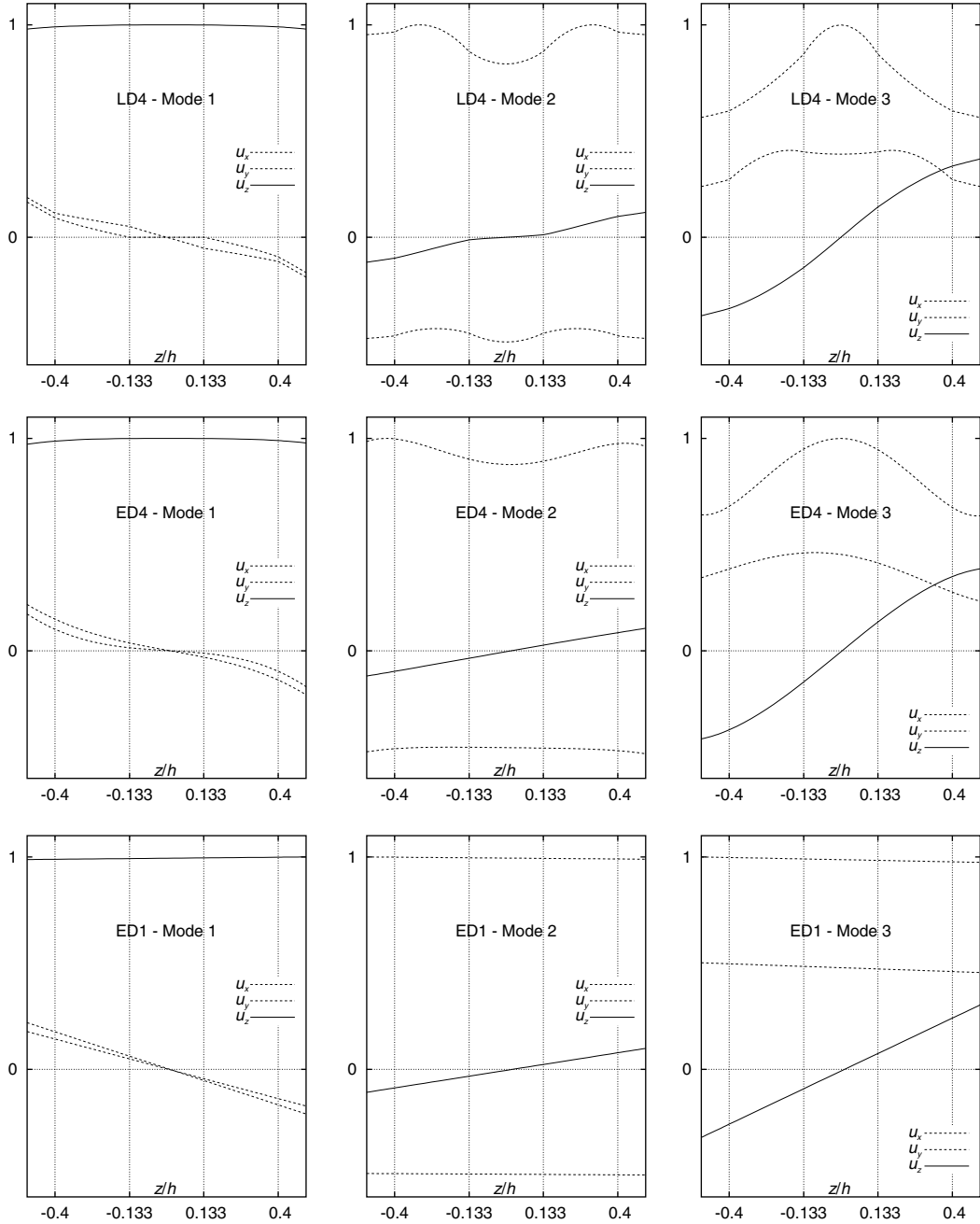
Fig. 12. Problem I, free vibration modes 1–3 of LD4, ED4 and ED1, al/h = 4 .
