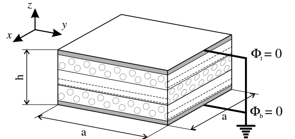
Fig. 7. Problem I, geometry and boundary conditions.
