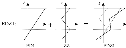
Fig. 3. Displacement assumptions of EDZ1.
