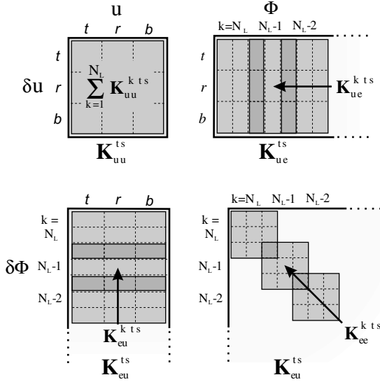
Fig. 6. ESL assembly of laminate arrays \mathbf{K}_{ij}^{ts} ( i, j = u, e ).
