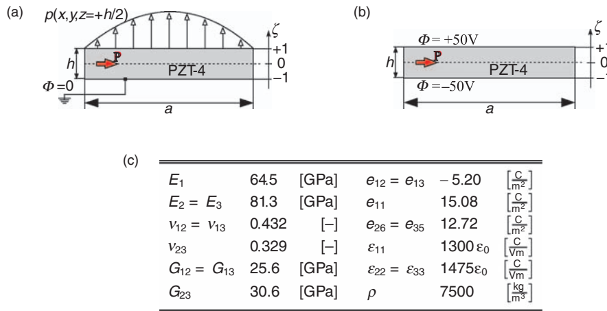
Figure 12. Piezoelectric plate working in 15-mode (shear mode): schematic of sensor and actuator configurations (top) and employed material data for PZT-4 (bottom). The polarization vector \mathbf{P} is taken parallel to the x -axis: (a) Sensor configuration; (b) Actuator configuration; (c) Material data for PZT-4 poled along x -axis ( \epsilon_0 = 8.854 \cdot 10^{-12} C/Vm).
