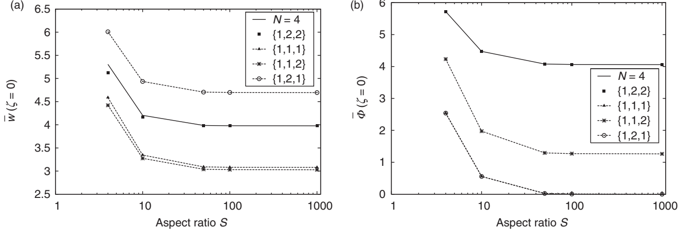
Figure 3. Piezoelectric sensor plate in 31-mode: non-dimensional global electromechanical response at the plate center for different aspect ratio S = a/h ( h = \text{constant} ): (a) Normalized deflection \bar{w}(\zeta=0) ; (b) Normalized electric potential \bar{\Phi}(\zeta=0) .
