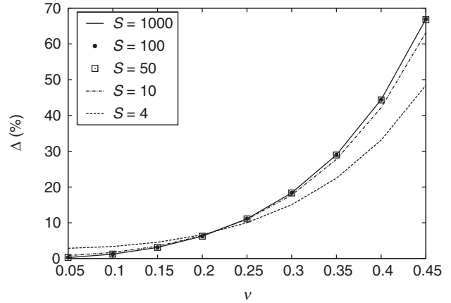
Figure 1. Percentage error on the transverse deflection for the model based on Reissner–Mindlin kinematics \{1, 0\} and full 3D constitutive law: influence of Poisson’s ratio \nu and aspect ratio S = a/h .
