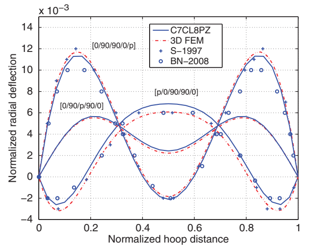
Figure 13. Simply supported 90° composite shell panel: effect of thickness location of the actuator.
