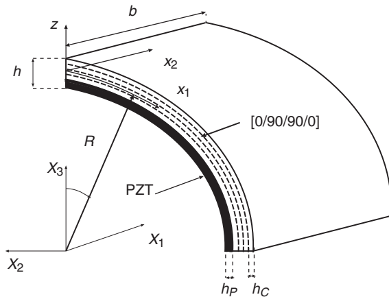
Figure 12. The 90° cylindrical panel [p/0/90/90/0]: a composite elastic laminate with a PZT actuator ( p ) attached to the inner (bottom) surface.
