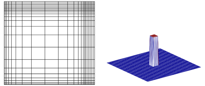
Fig. 10. Mesh N_x = N_y = 22 sr(14) (left) – localized pressure (right).
