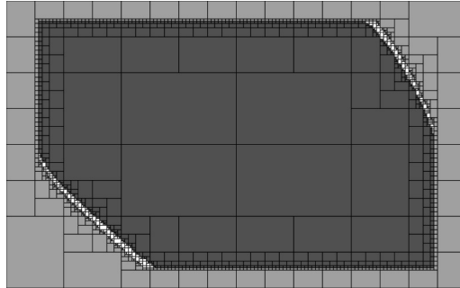
Figure 6: Approximations of the viability kernel.
