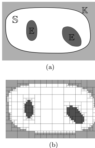
Figure 2: Subpaving representing the initial inner approximation for \text{Viab}_{\mathcal{S}}(\mathbb{K})
