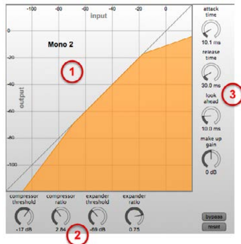
Figure 2. Compressor/expander module. ① Dynamic compression curve. ② Ratios and thresholds. ③ Temporal characteristics.
