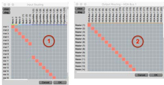
Figure 5. ① Input routing. Physical inputs (rows of the matrix) can be assigned to the available tracks (columns). ② Panning bus routing “HOA 1”. The output of the bus (columns) can be routed to the Master channels (rows), i.e. towards the physical outputs. Each channel can have multiple connections (e.g. one physical input can be routed to several tracks).
