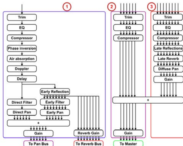
Figure 7. Audio architecture (simplified representation). ① Mono track. ② Panning/decoding bus. ③ Reverb bus.
