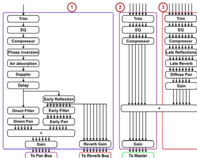
Figure 7. Audio architecture (simplified representation). ① Mono track. ② Panning/decoding bus. ③ Reverb bus.
