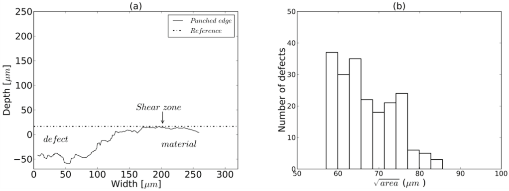
Fig. 7. (a) Reference for critical defect size calculation, (b) distribution of largest punching defects
