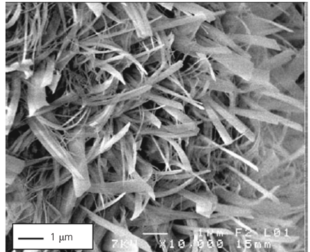
Figure 6. SEM micrograph of xonotlite morphology
