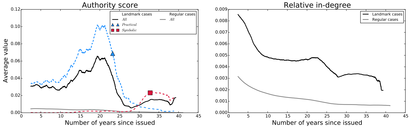
Fig. 2. Landmark vs. regular cases
